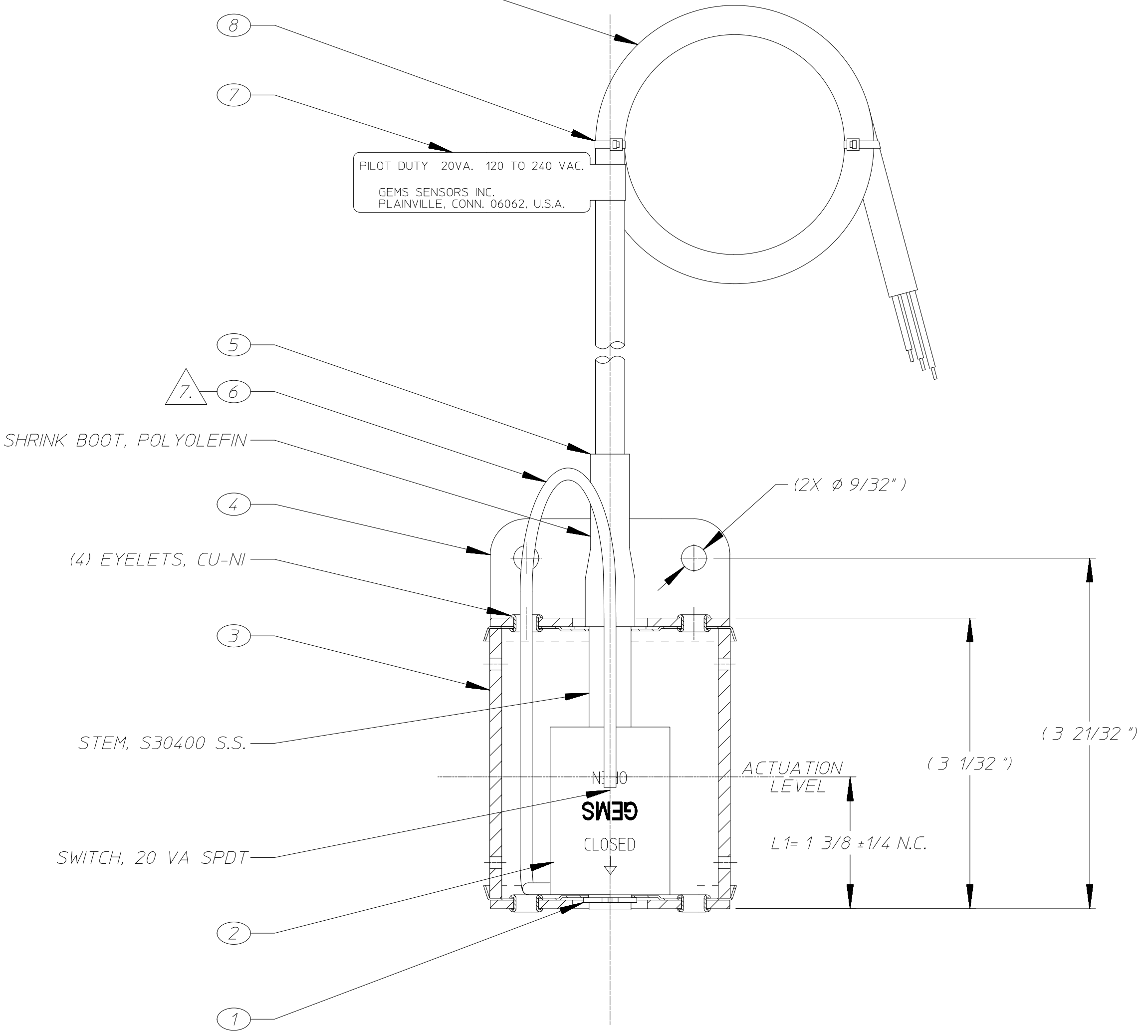
SECTION A~A
