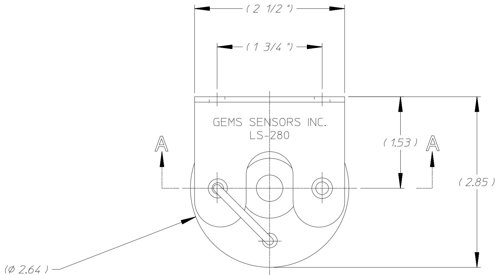
TOP VIEW (SHOWN W/O CABLE/STEM ASS'Y)
