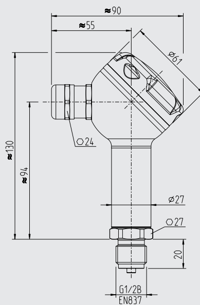
Field case Cable gland adjustable
