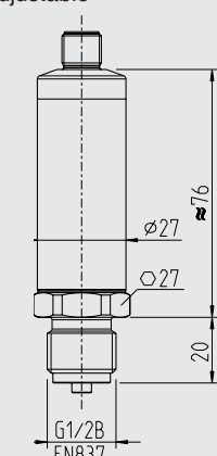
Circular connector M12 x 1 IEC 61076-2-101 A-COD (4-pin) not adjustable
