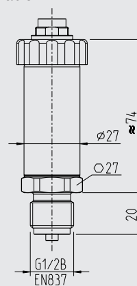
Circular connector M16 x 0.75 IEC 61076-2-106 (5-pin) adjustable
