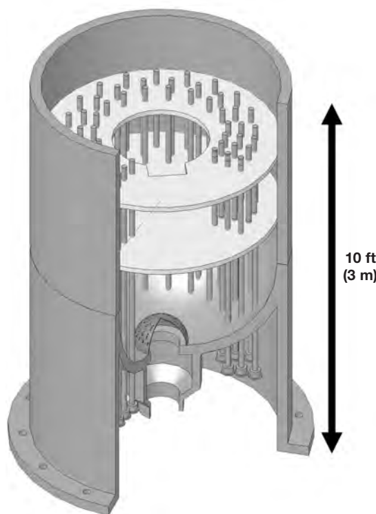
Nuclear Pressurizer Heaters
