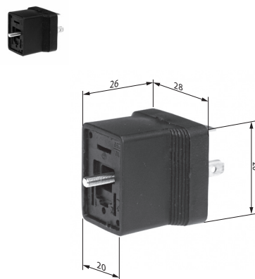
Type 02 Adapter from form A to form B
