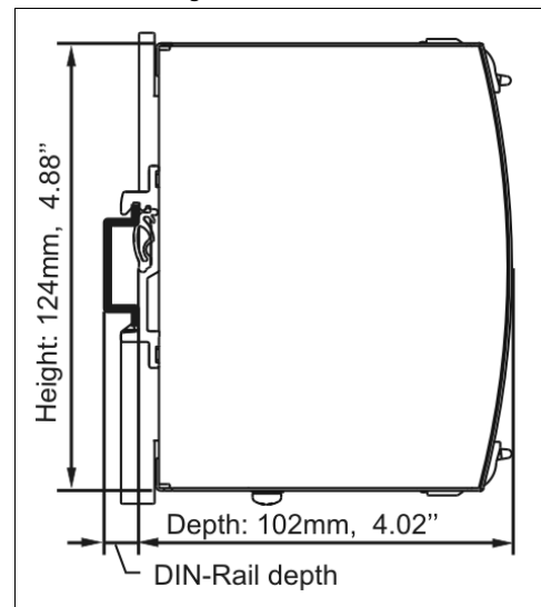
Fig. 19-2 Side view
