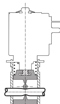
2/2 Normally Open
