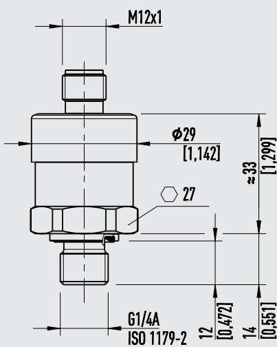
With circular connector M12 x 1
