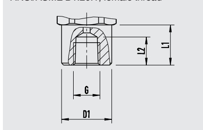
ANSI/ASME B1.20.1, female thread
