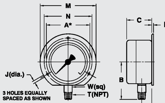
LM/REAR FLANGE
