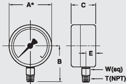
LOWER MOUNT
