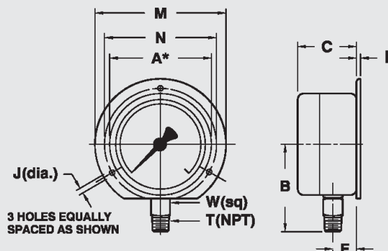
LM/REAR FLANGE
