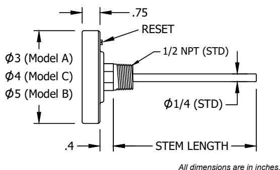
Standard Dimensions
