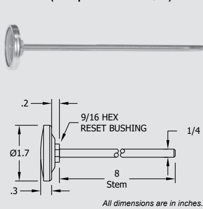
Lab Model GL with 1.7" Dial (with point - Model GLP)
