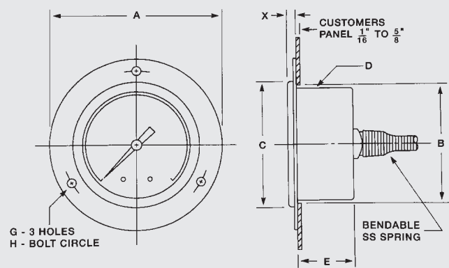
Front Flange Case Dimensions
