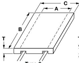
Type 6 Insulated Sides (Style B Leads Illustrated)
