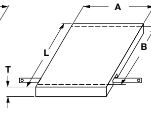
Type 7 Insulated Ends (Style C Leads Illustrated)
