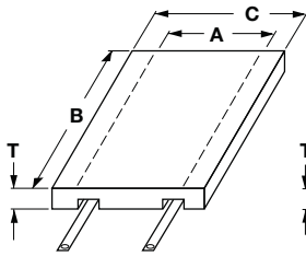
Type 6 Insulated Sides (Style B Leads Illustrated)
