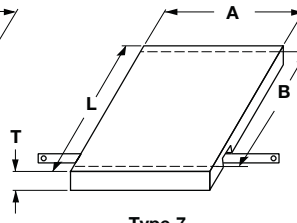
Type 7 Insulated Ends (Style C Leads Illustrated)
