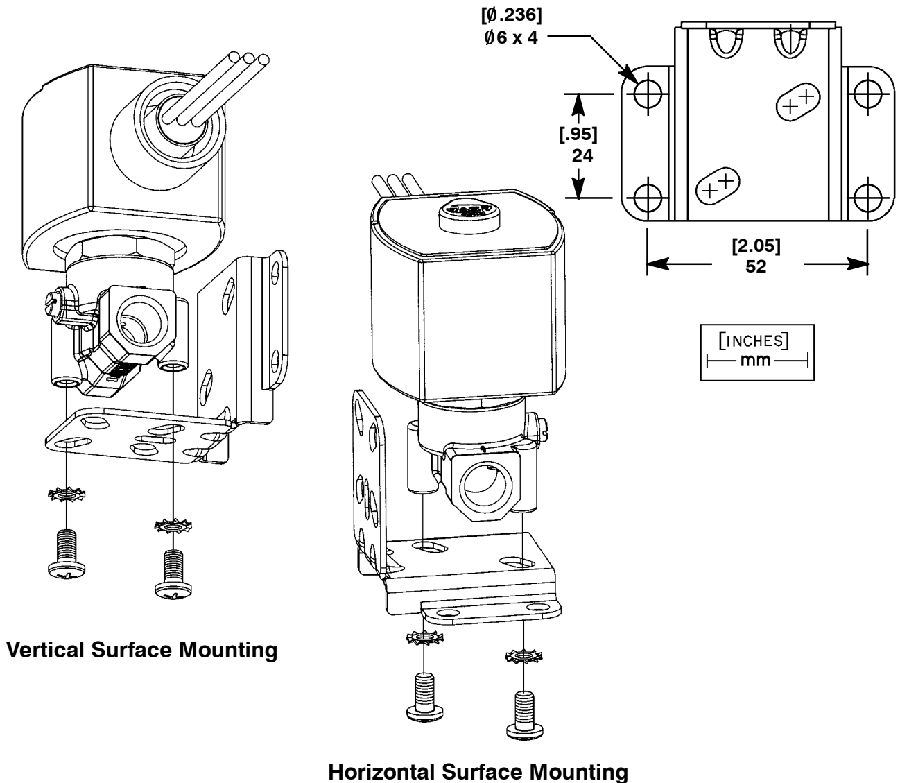
Fig. 1. Mounting Bracket
